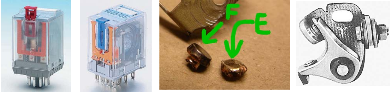
Pic 10, 11, 12 and 13. Industrial relays and contact surfaces. E is the old surface and F is the new. Breaker for car.
