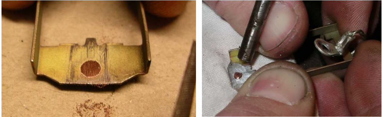
Pic 8 and 9. The backside of the contact surface is filed off so the removal of the surface went smoothly. The new surface is mounted in the hole from the old one and riveted with a mandrel. Be careful not to damage the surface.
