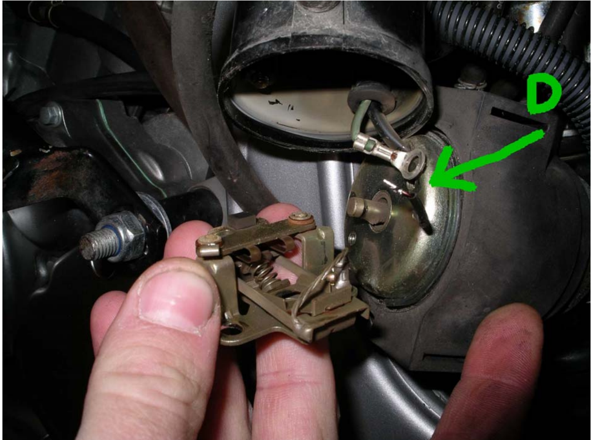
Pic 14. Switch loosened. D shows unsoldered wire.
