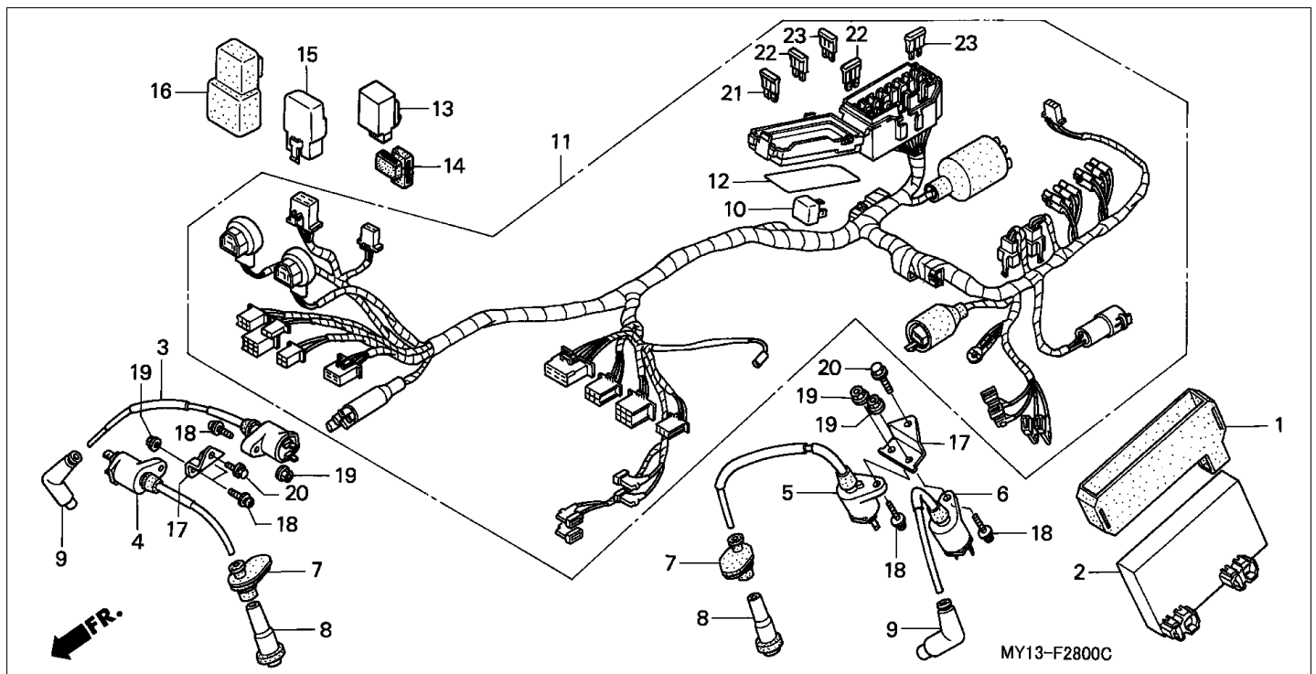
Block F-28 WIRE HARNESS/ IGNITION COIL (1)
